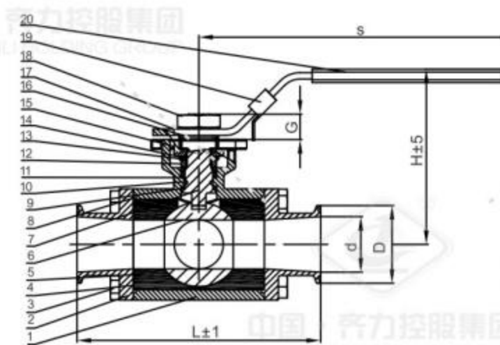
1/2"-4"Encapsulated and ISO mounting pad. Mounting pad connection size please refer to the standard ISO5211
