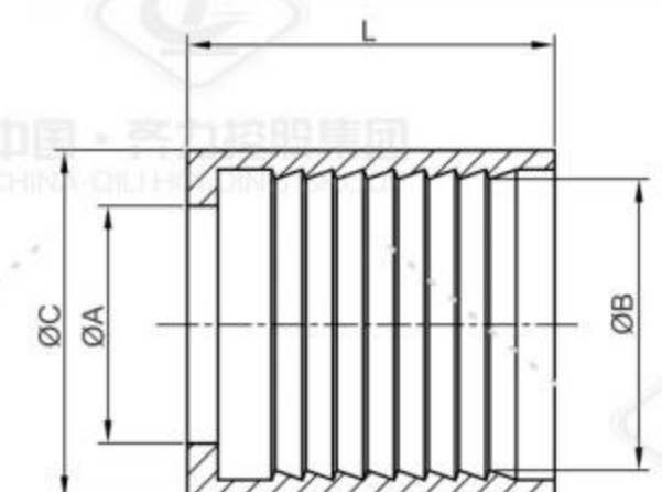
软管接头套筒 Hose crimp
