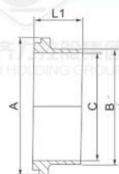
焊接接头 Welded ferrule
