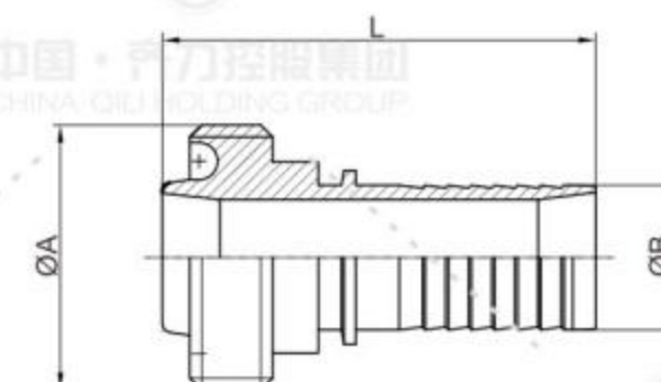
RJT公头扣压接头 RJT Male hose adapter
