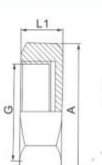
六角盲盖 Hexagonal blind ferrule
