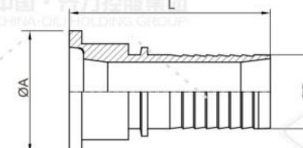
RJT母头扣压接头 RJT Female hose adapter
