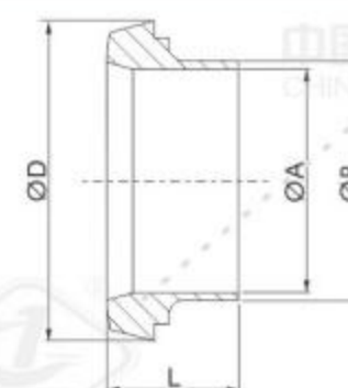
DIN-151IIMPERIAL WELDING MALE
