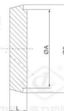
DIN-15 DA/DB WELDING LINER
