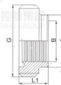
膨胀型螺纹接 Expanding male
