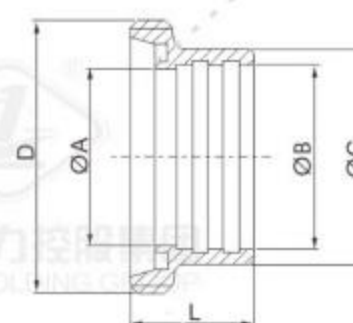
DIN-15R EXPANDING WELDING MALE
