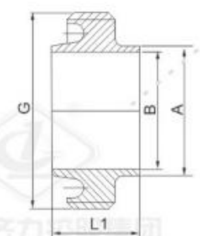
螺纹接头 Threaded ferrule
