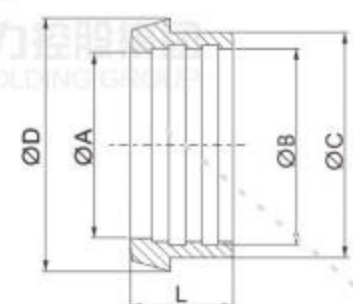
DIN-14 WELDING LINER
