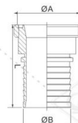
SMS软管接头 SMS hose adapter
